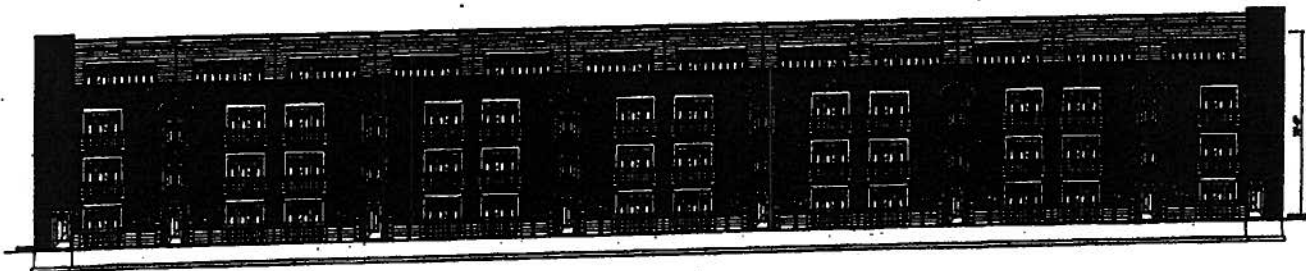
TYPICAL 4 STORY MASONRY BLDG. (24 DU)-FRONT ELEVATION
