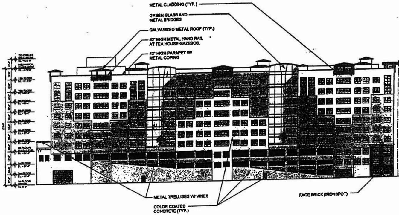
WEST ELEVATION
