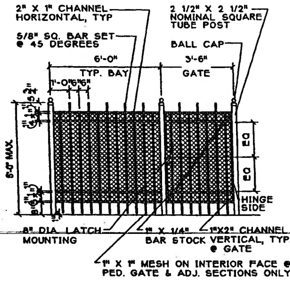
TYP. ORNAMENTAL IRON FENCE
