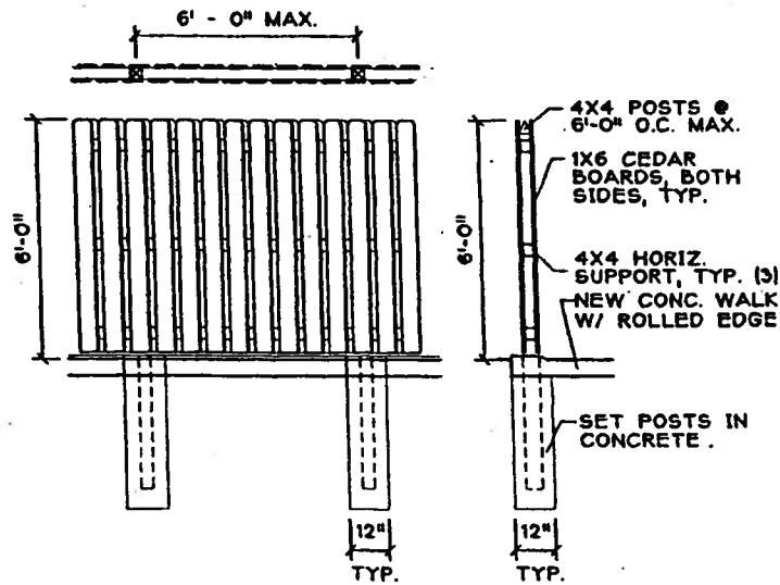
TYP. BOARD ON BOARD WD. FENCE
