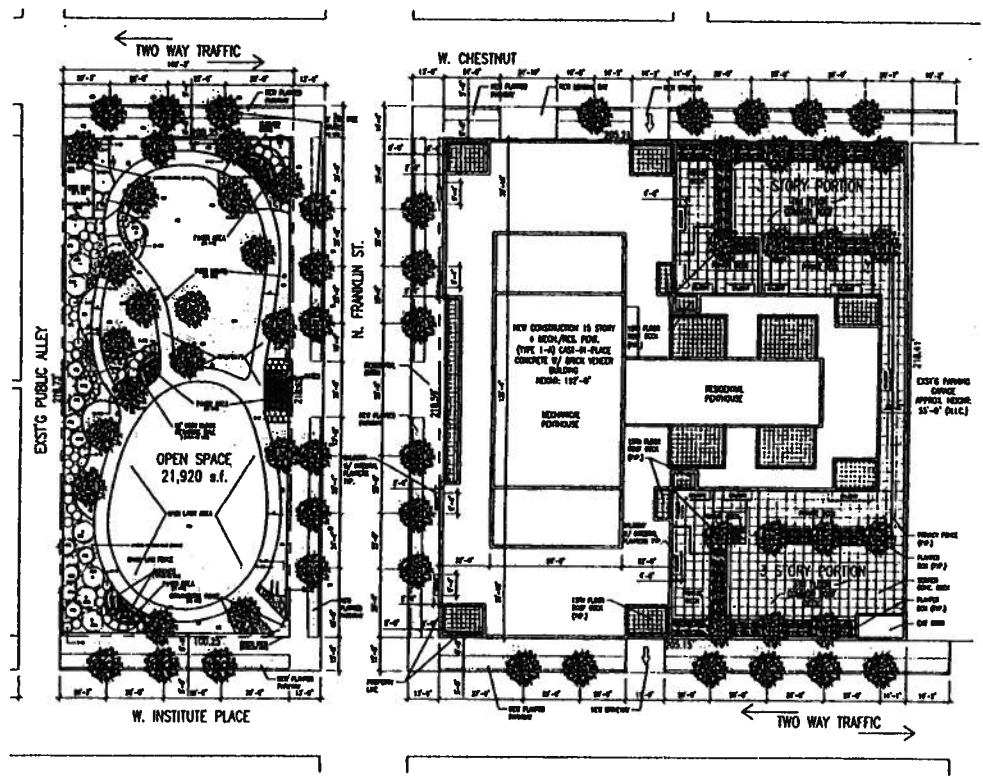
1 SITE PLAN 1"=20'-0"
