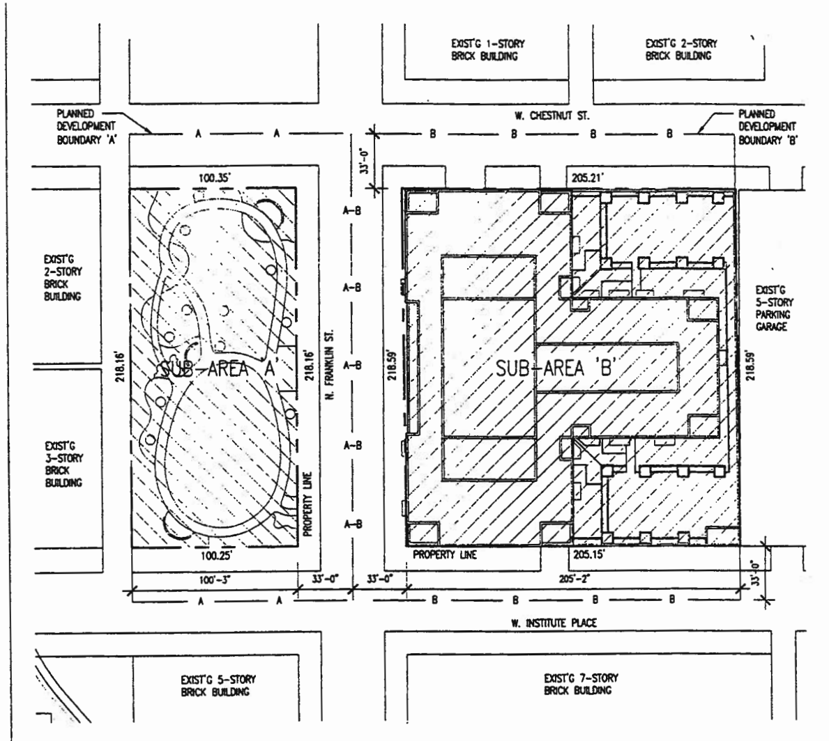
1 PLANNED DEVELOPMENT BOUNDARY, PROPERTY LINE & SUB-AREA MAP SCALE: 1/64" = 1'-0"
