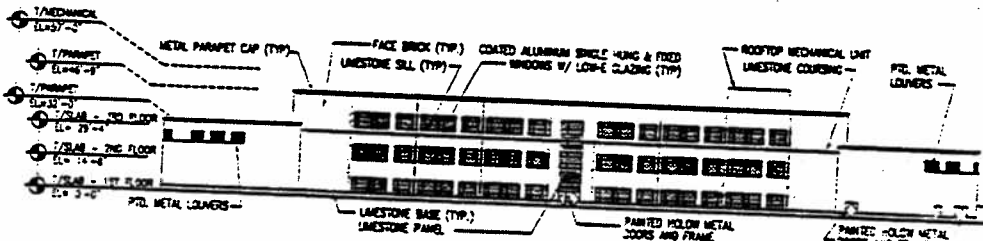
WEST ELEVATION
