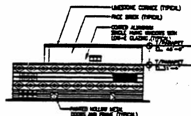
EAST ELEVATION
