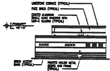
SOUTH ELEVATION
