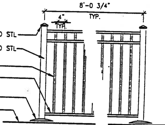
TYPICAL FENCE ELEVATION
