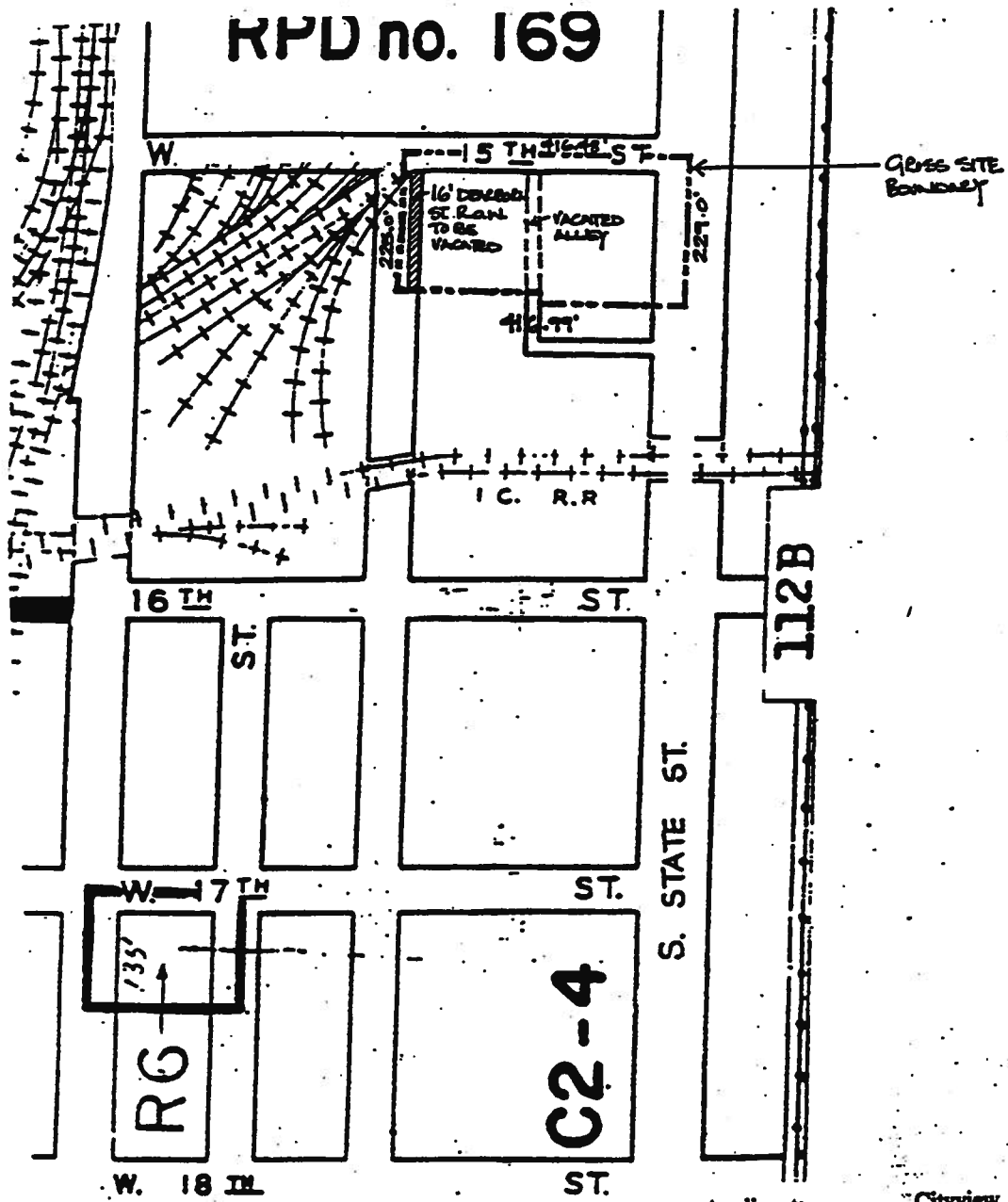
PLANNED DEVELOPMENT PROPERTY LINE, BOUNDARY AND R.O.W. ADJUSTMENT MAP.
