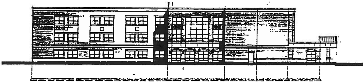
NORTH ELEVATION
