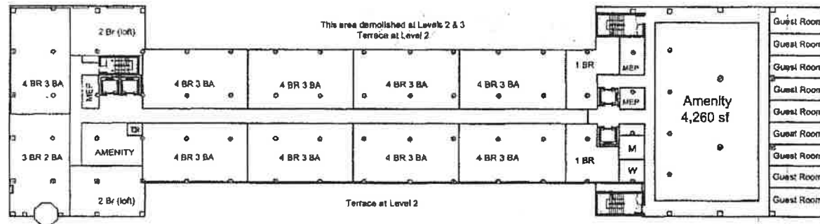
Levels 2&3 Plan
