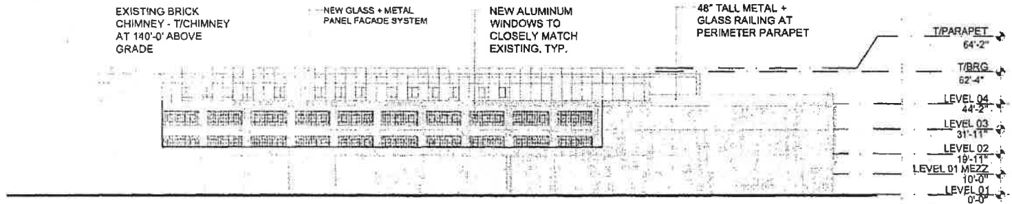
South Elevation
