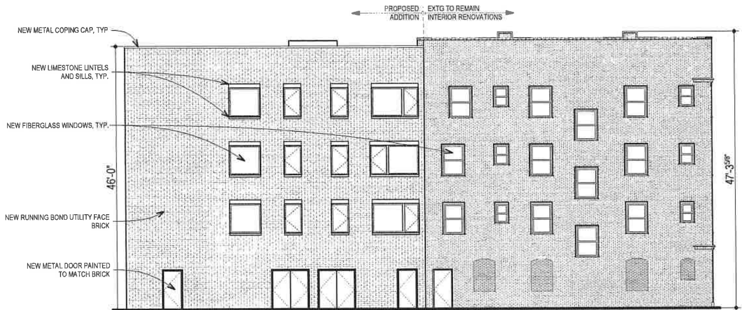
South Elevation - Alley
