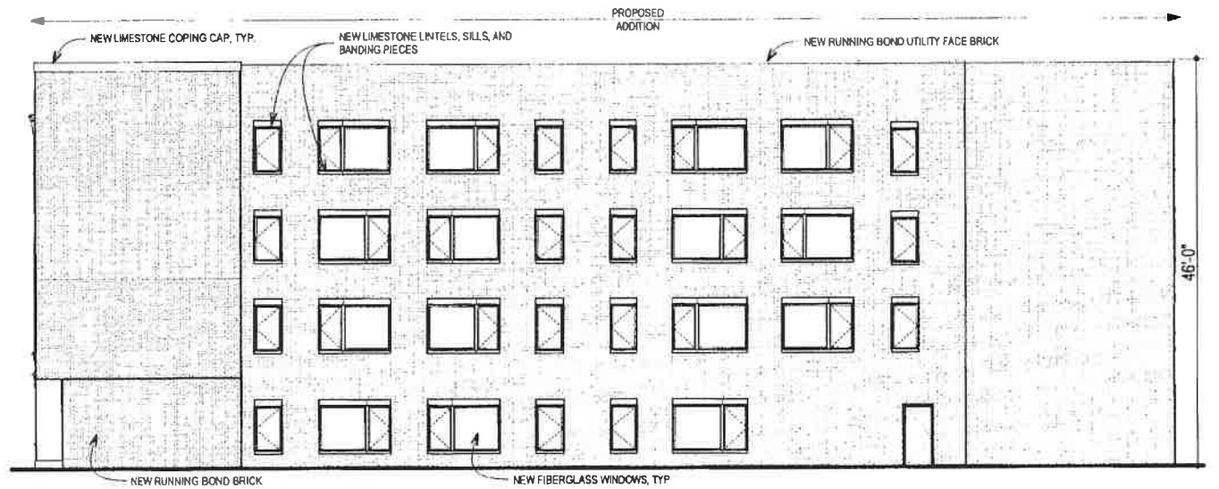
West Elevation - Interior Lot Line
