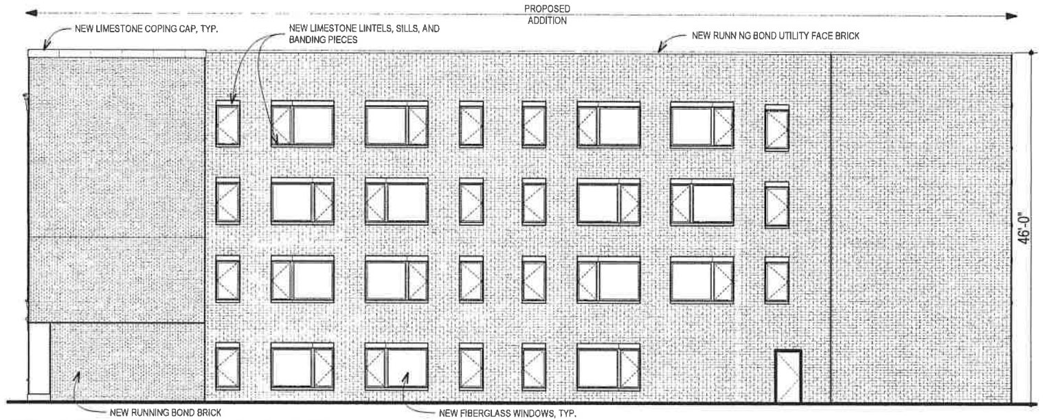
West Elevation - Interior Lot Line
