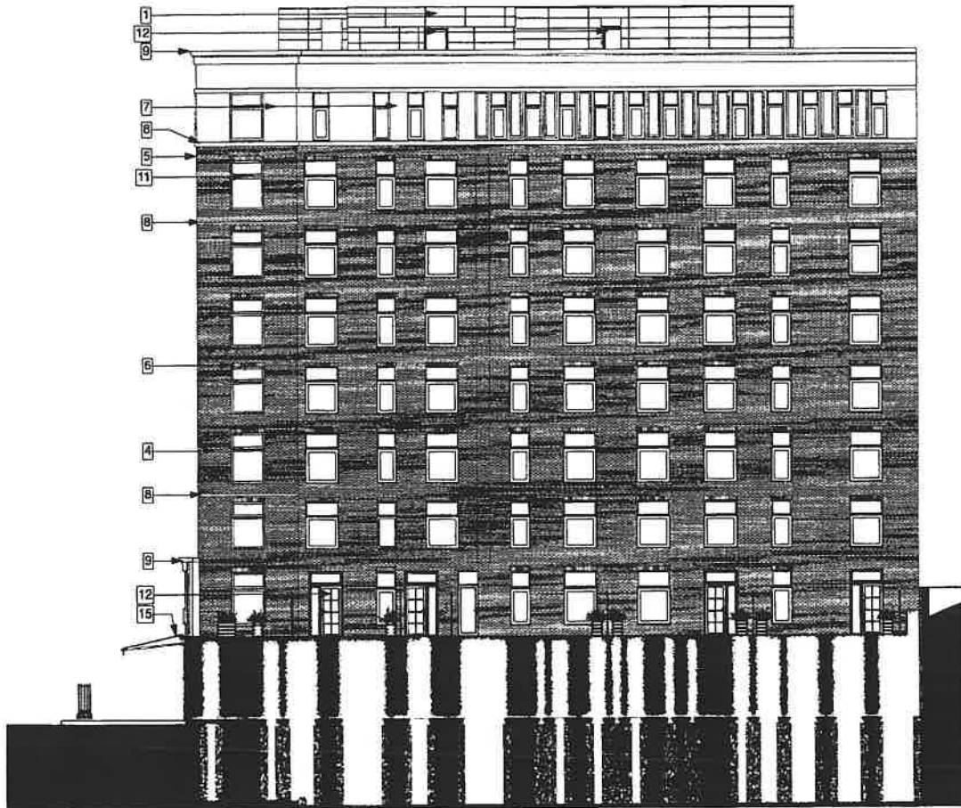
Refer to Building Section for vertical height information.
