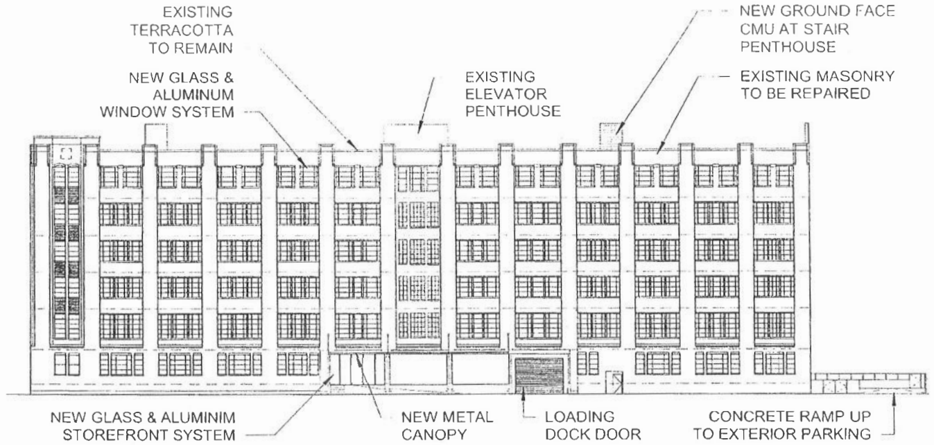
WEST ELEVATION
