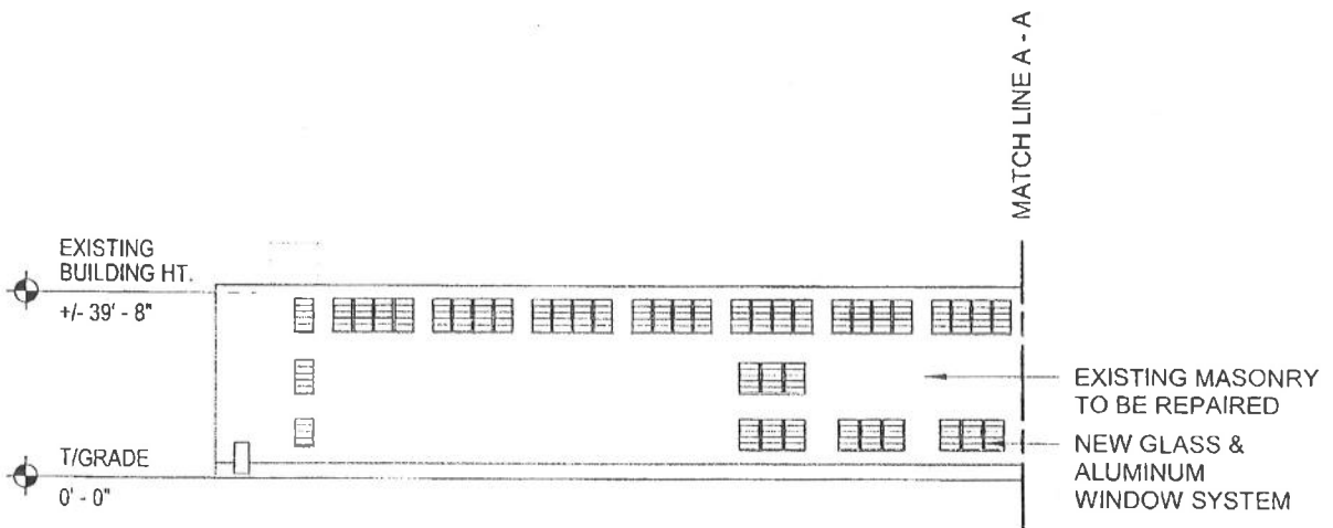
EAST ELEVATION - NORTH PORTION
