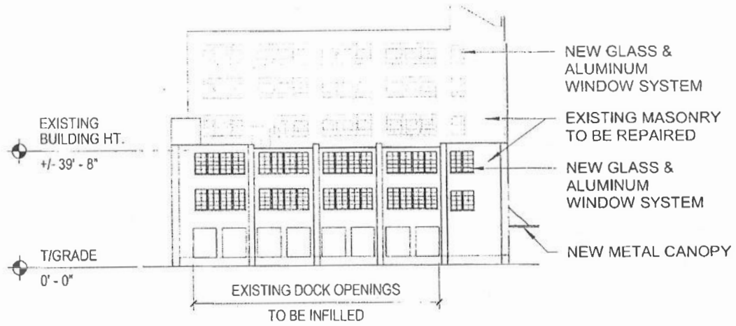
SOUTH ELEVATION
