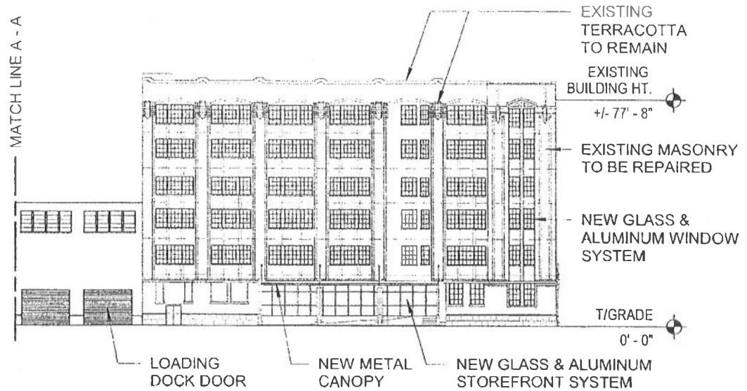
EAST ELEVATION - NORTH PORTION
