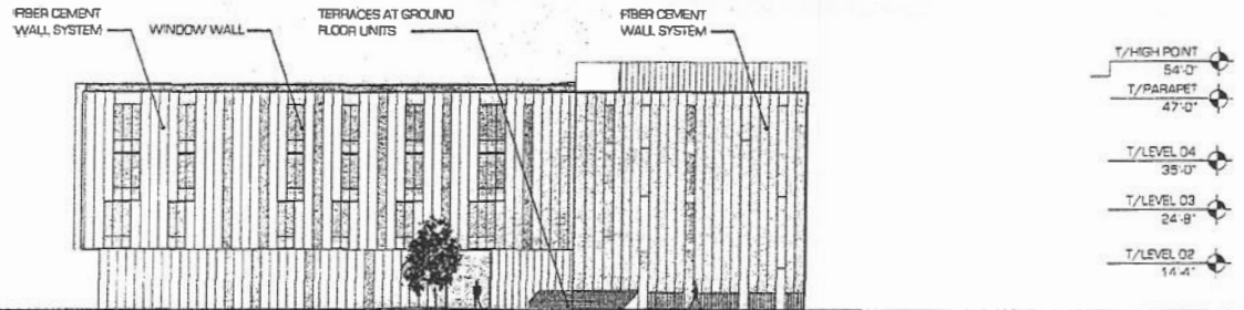
SOUTH ELEVATION
