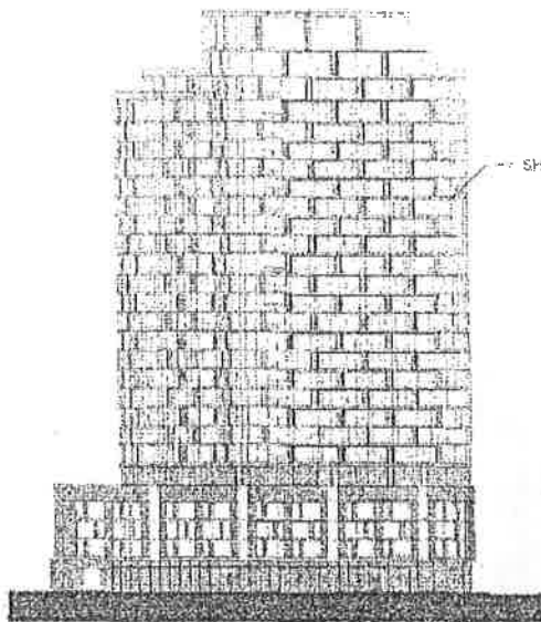
SOUTH ELEVATION
