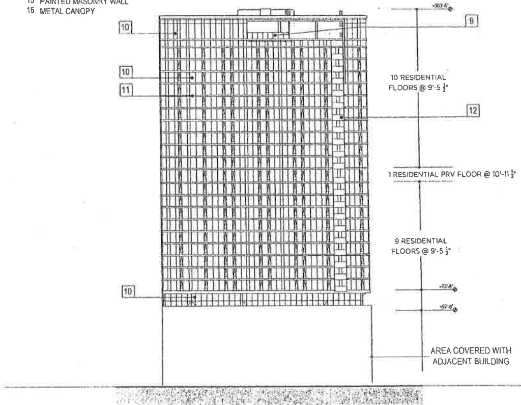
NORTH ELEVATION
