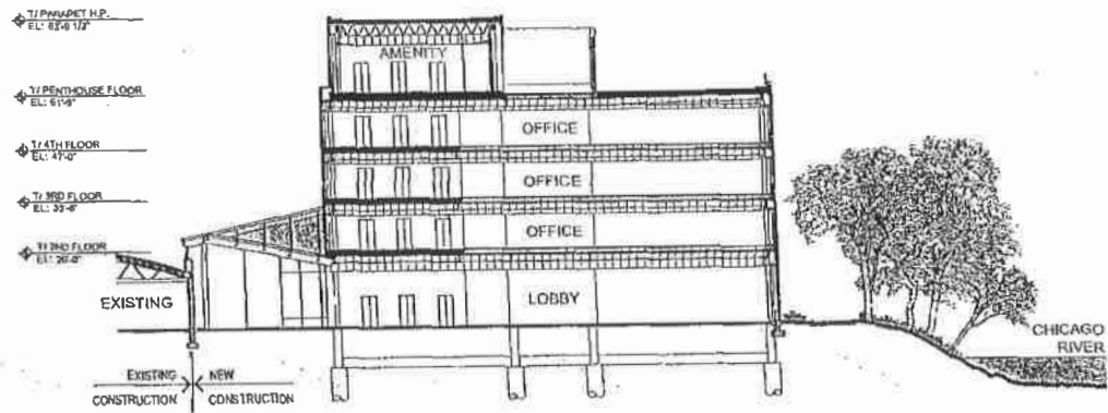
BUILDING SECTION
