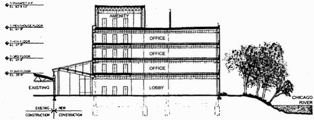
BUILDING SECTION
