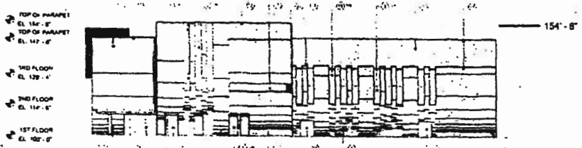
WEST ELEVATION
